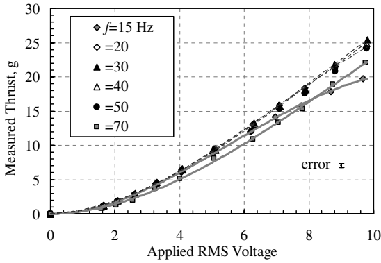
Fig. 7 Measured, time-averaged jet thrust as function of RMS speaker voltage.
