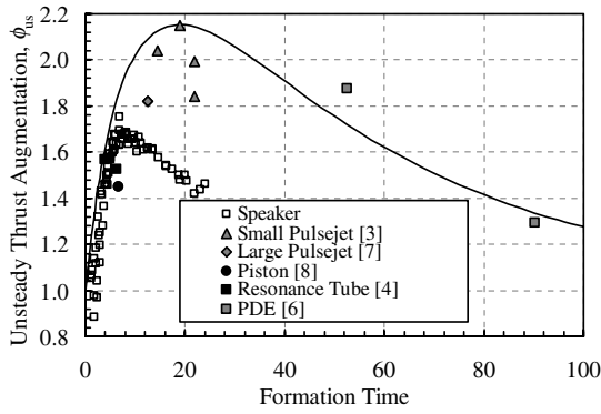
Fig. 12 Unsteady thrust augmentation as function of formation time for tested thrust sources.
